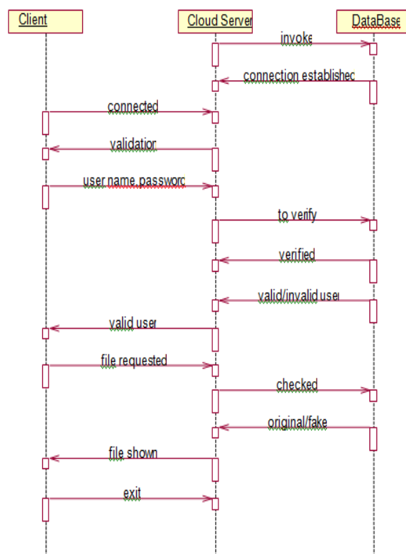
Figure 5.3: Sequence Diagram
